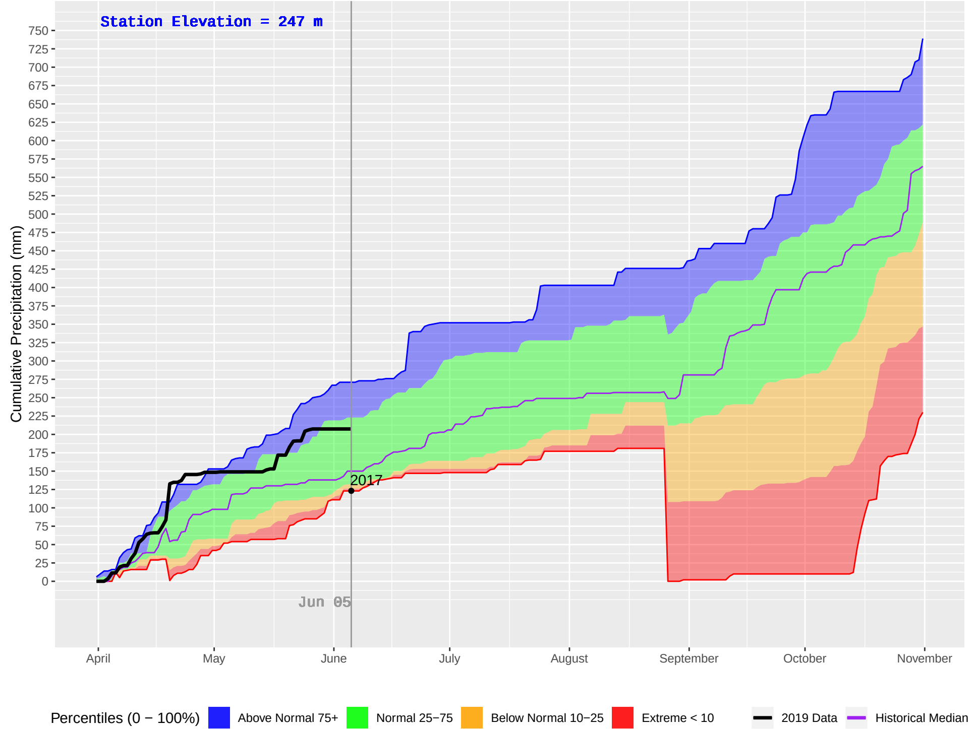
FORD MOUNTAIN (1144) : Historical (2012–2018), Current (2019) Daily Cumulative Precipitation
