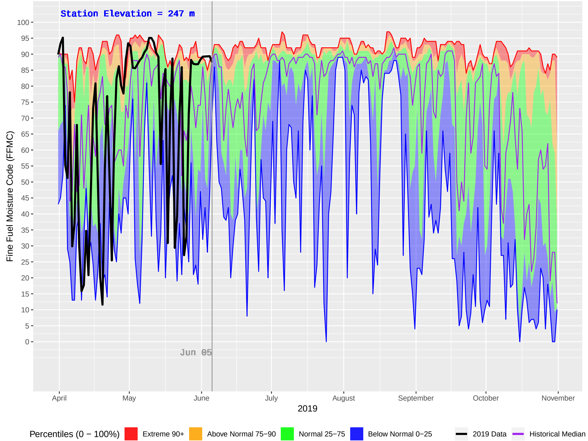
FORD MOUNTAIN (1144) : Historical (2012–2018) and Current (2019) Daily Fine Fuel Moisture Code (FFMC)
