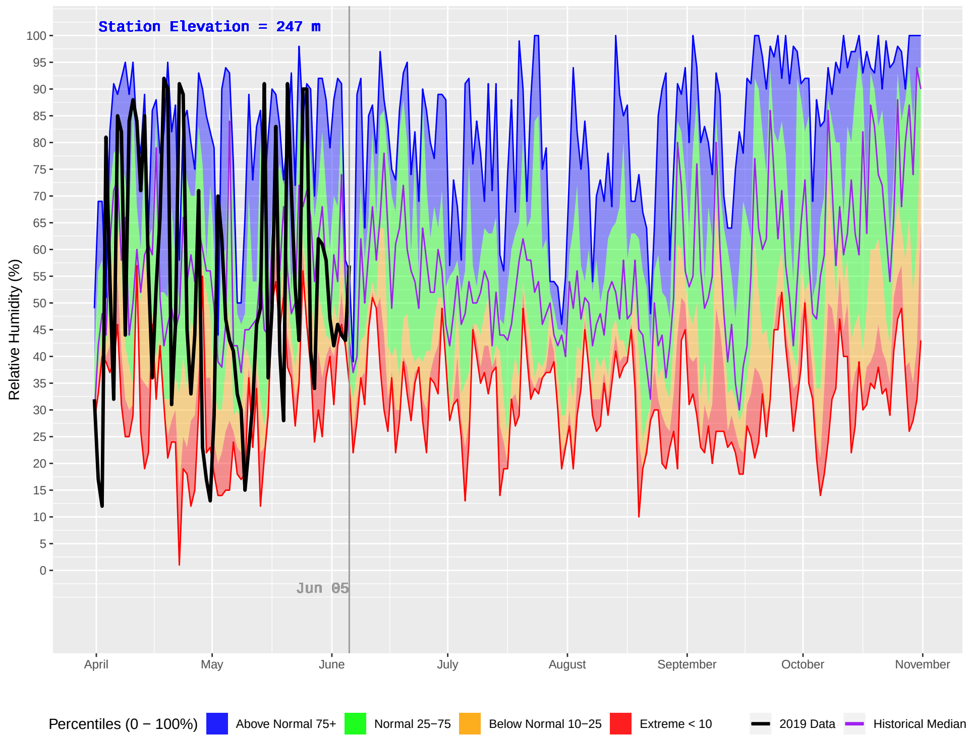
FORD MOUNTAIN (1144) : Historical (2012–2018) and Current (2019) Daily Relative Humidity
