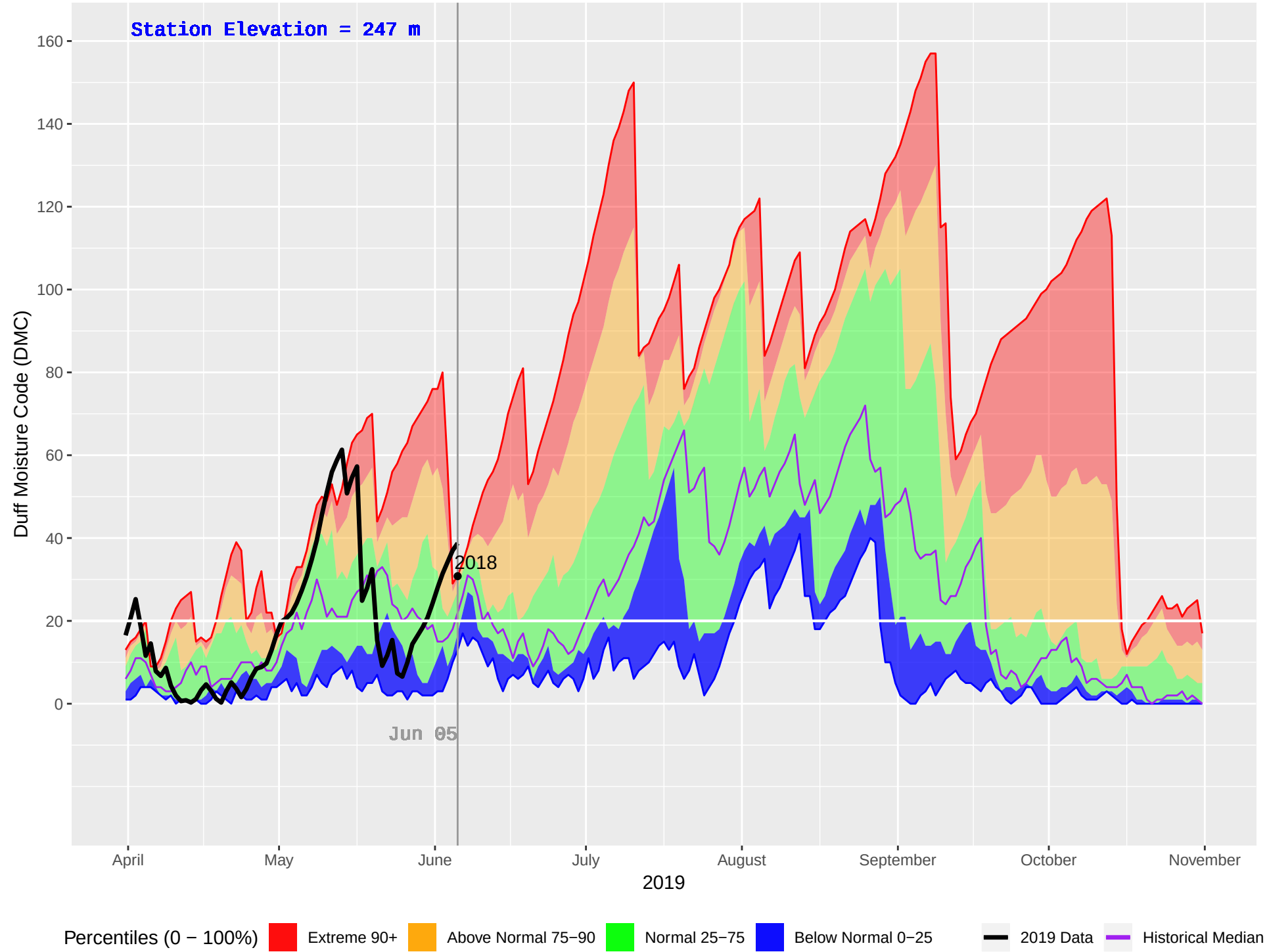
FORD MOUNTAIN (1144) : Historical (2012–2018), Current (2019) Daily Duff Moisture Code (DMC)
