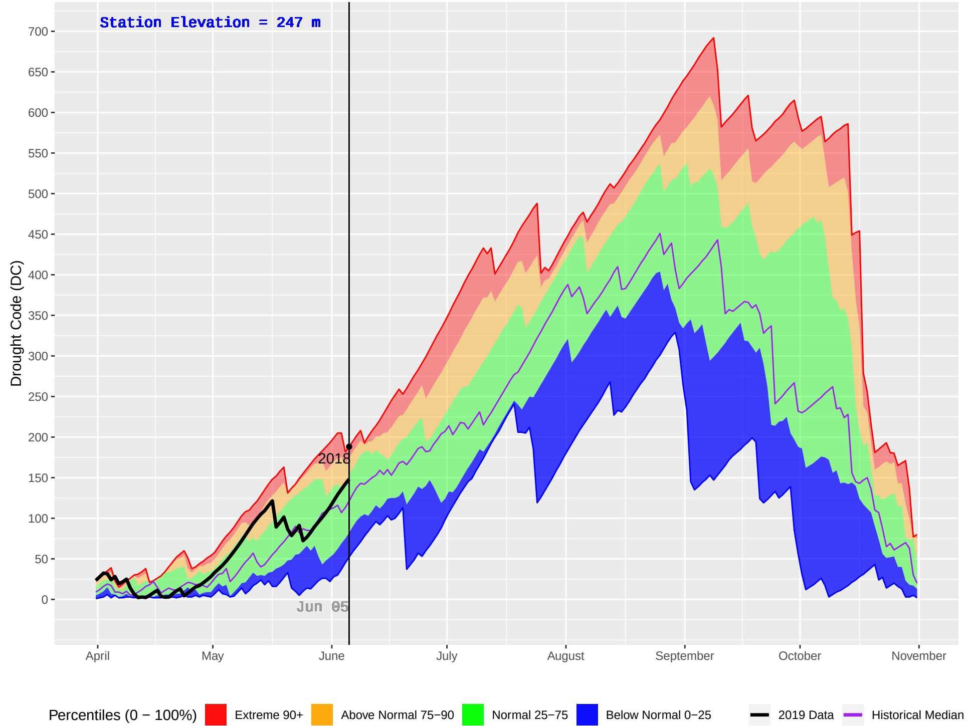
FORD MOUNTAIN (1144) : Historical (2012–2018) and Current (2019) Daily Drought Code (DC)
