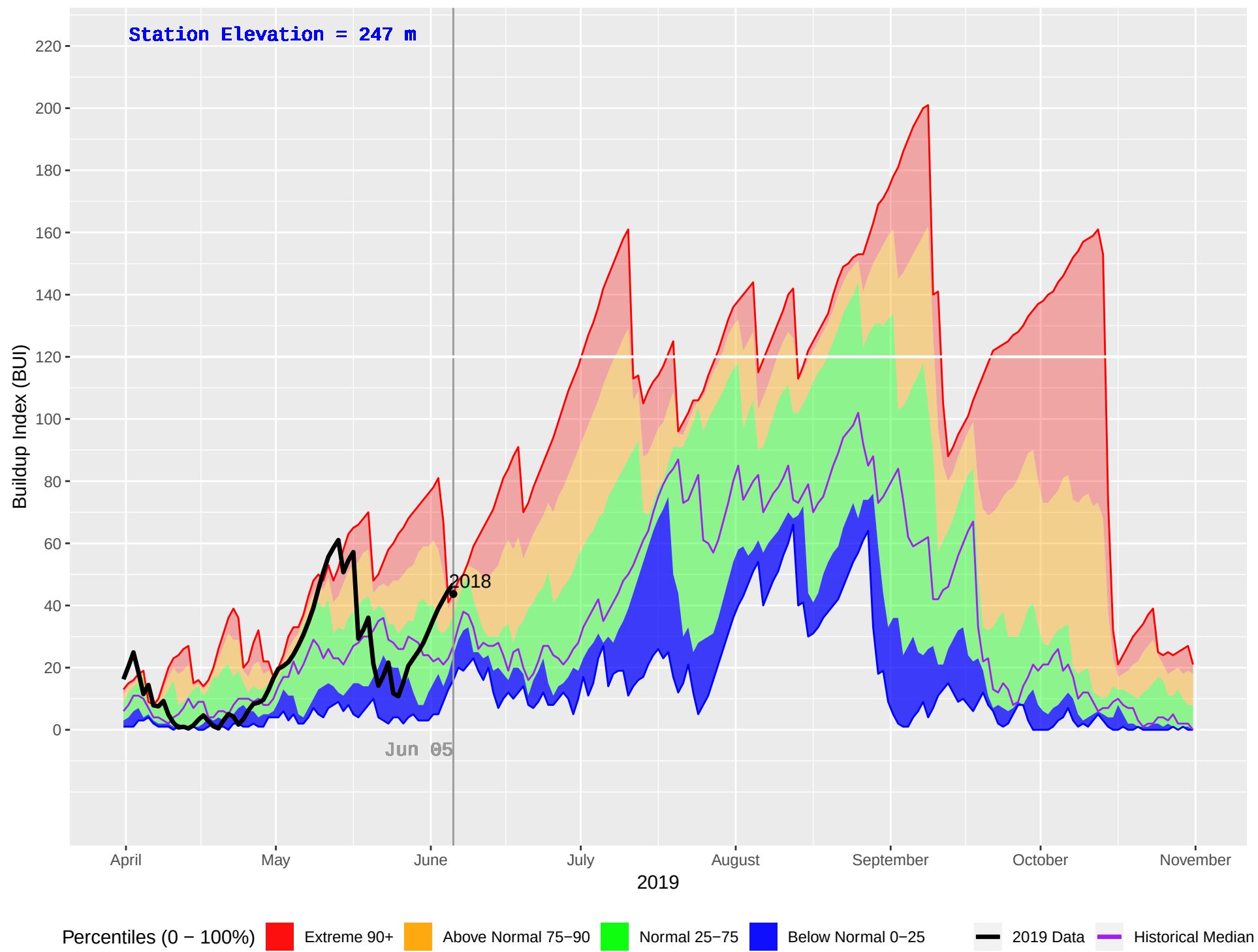
FORD MOUNTAIN (1144) : Historical (2012–2018), Current (2019) Daily Buildup Index (BUI)
